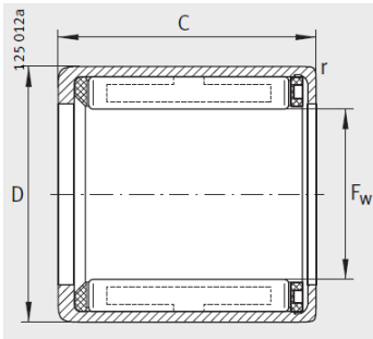
HF、HF..-KF
